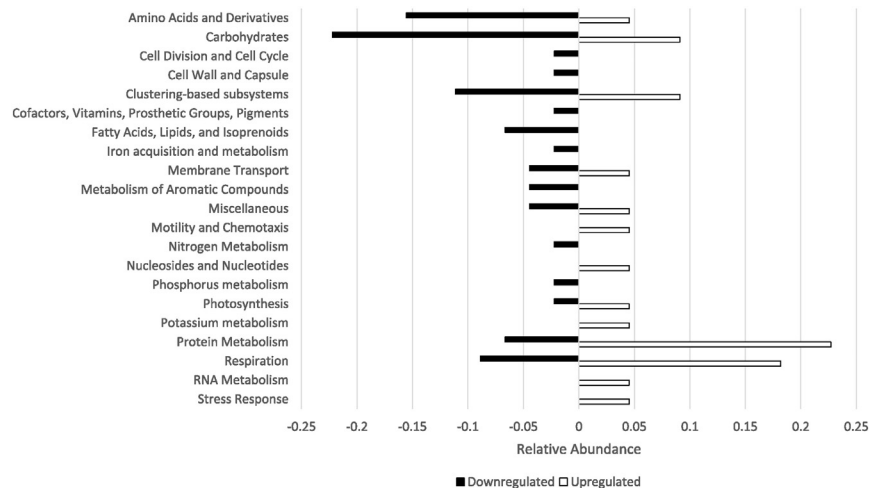
Fig. 3. Relative abundance of SEED functional roles down- and up-regulated in response to glyphosate treatment sorted by SEED Level 1 subsystem classifications. Relative abundance was estimated as the proportion of functional roles within a given Level 1 subsystem relative to the total number of functional roles down- or up-regulated.
